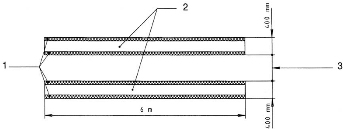
Drawing of the rolling track
